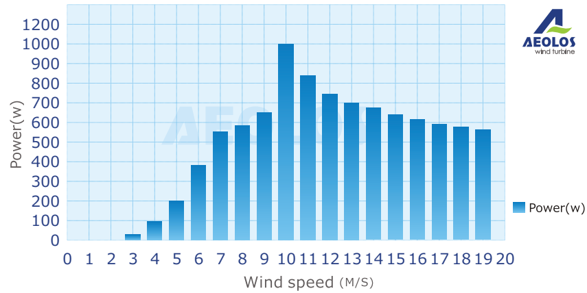
Wind Speed/ Power Curve
