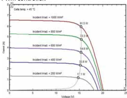
Figure 16: Dependence of M_p and V_{mp} on irradiance
